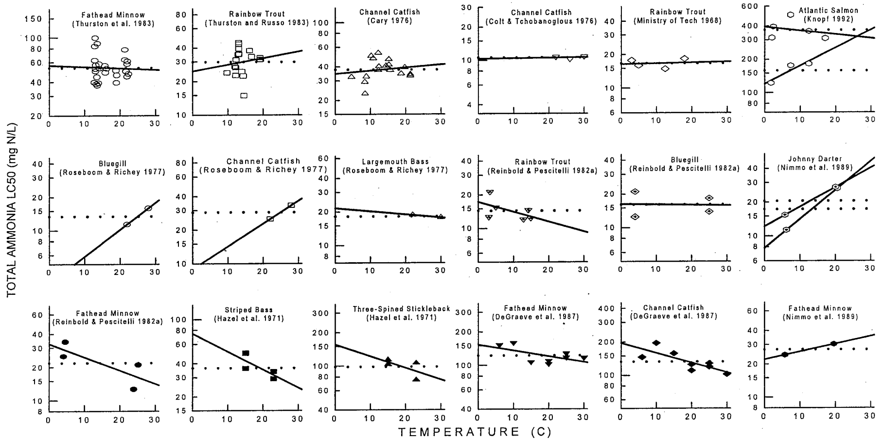
Figure 3. The effect of temperature on pH-adjusted acute ammonia toxicity in terms of total ammonia. LC50s are adjusted to the mean pH of the dataset based on the pooled relationship of acute toxicity to pH. Symbols denote LC50s, solid lines denote regressions for individual datasets, and dotted lines denote pooled regression over all datasets.
